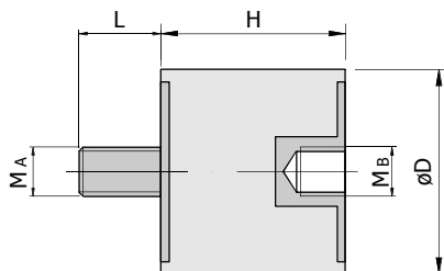
Nosač gumeni Tip-C \varnothing D \times H ; M_A \times L / M_B
