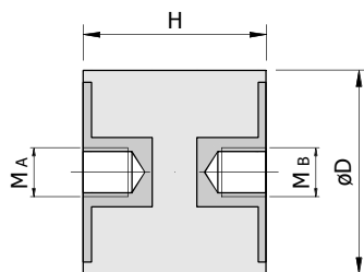
Nosač gumeni Tip-B \varnothing D \times H ; M_A / M_B
