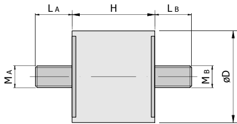
Nosač gumeni Tip-A \varnothing D \times H ; M_A \times L_A / M_B \times L_B
